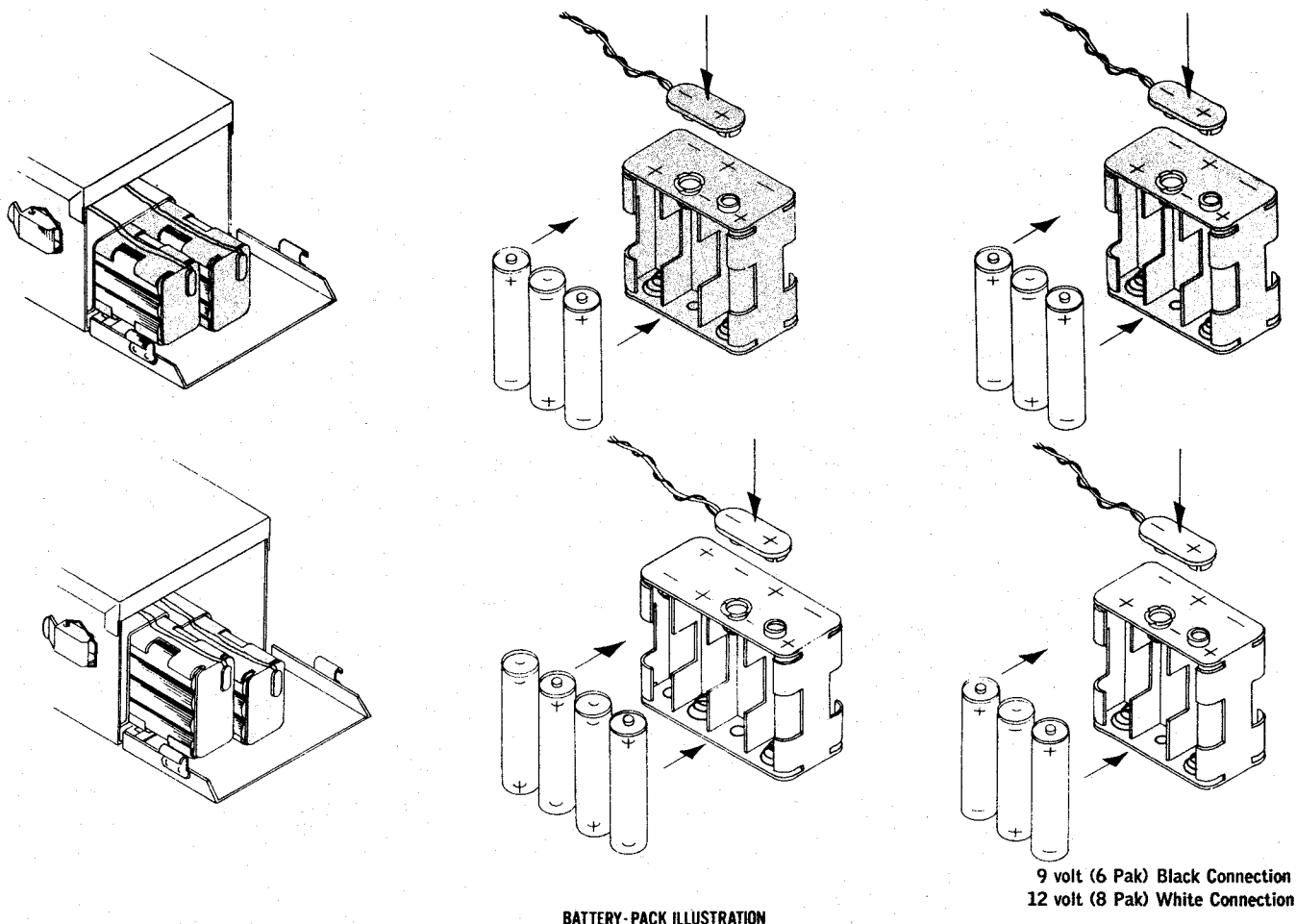
BATTERY-PACK ILLUSTRATION
